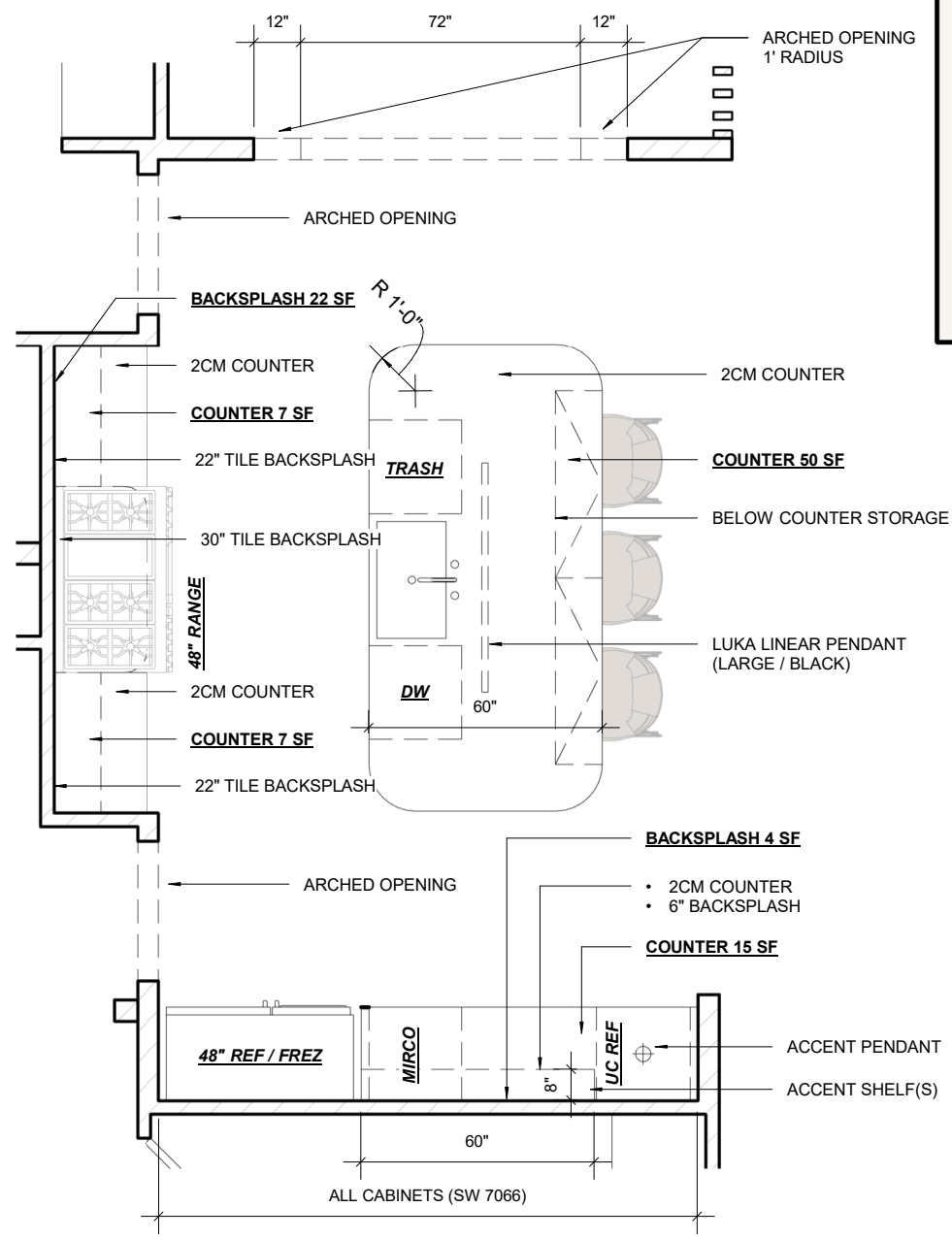
1 ID PLAN AT KITCHEN 1/4" = 1'-0"
